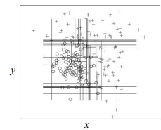
Decision boundary of the 10 trees used by AdaBoost
