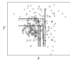
Decision boundary of the 10 trees used by Bagging
